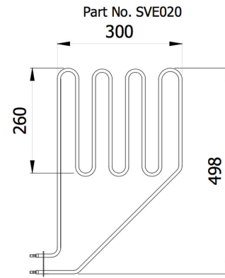
2000w Element Suits Helo SKLE and SKLA Heaters
